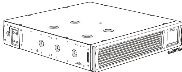
SMC1500-2UC e SMC1500I-2UC Montaggio a rack
